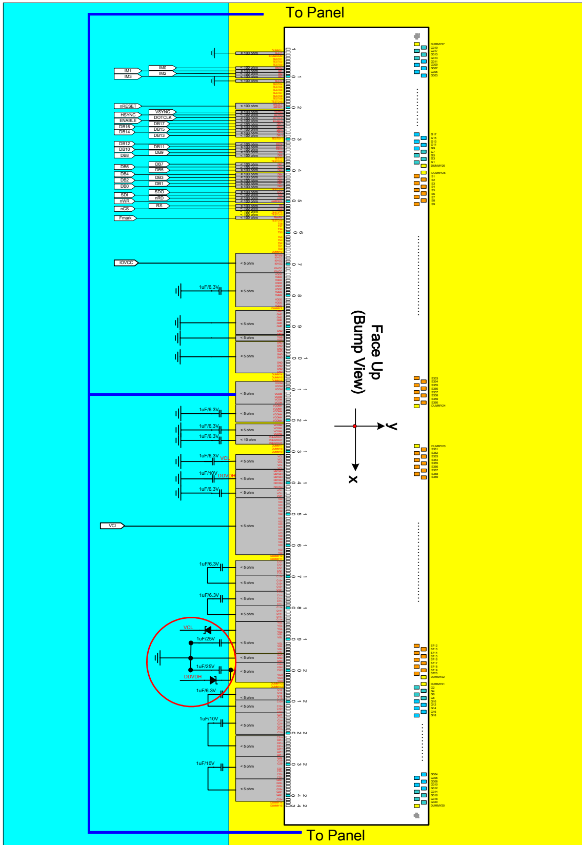
Figure 43 Power Supply Circuit Block
