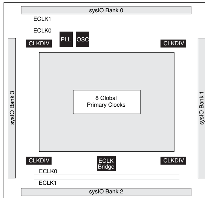
Figure 1. MachXO2 Clocking Structure (MachXO2-1200)
