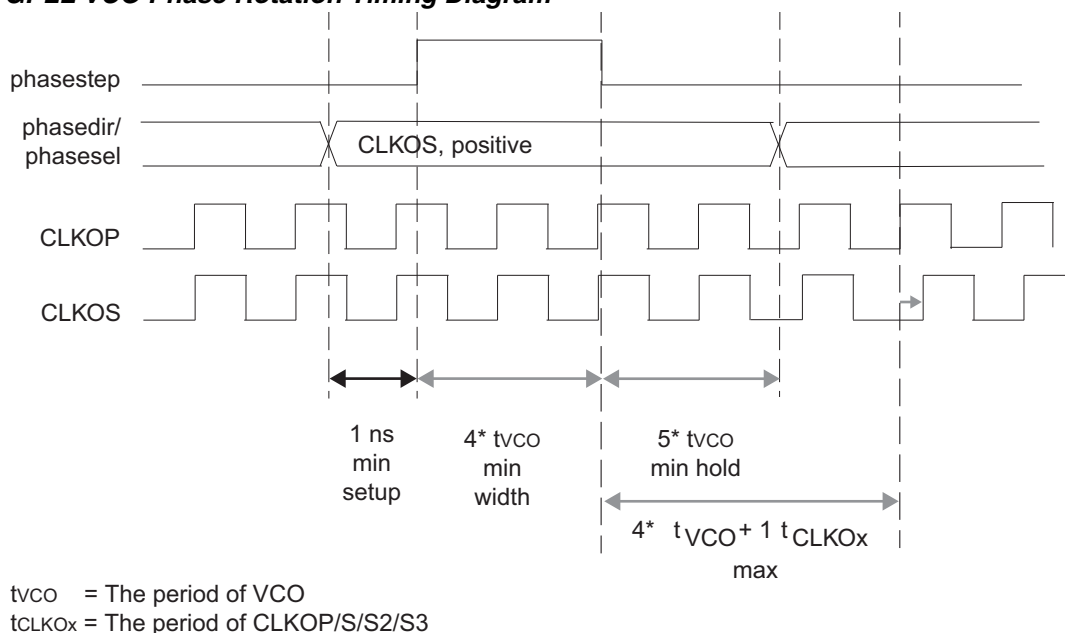
Figure 12. GPLL VCO Phase Rotation Timing Diagram
