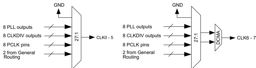
Figure 19. MachXO2 Primary Clock Muxes – MachXO-640U, MachXO2-1200/U and Higher Density Devices
