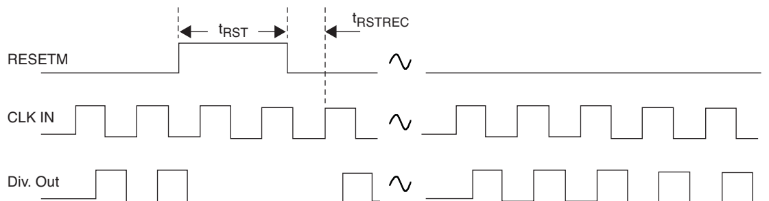
Figure 9. RST and RESETM Timing Diagram
