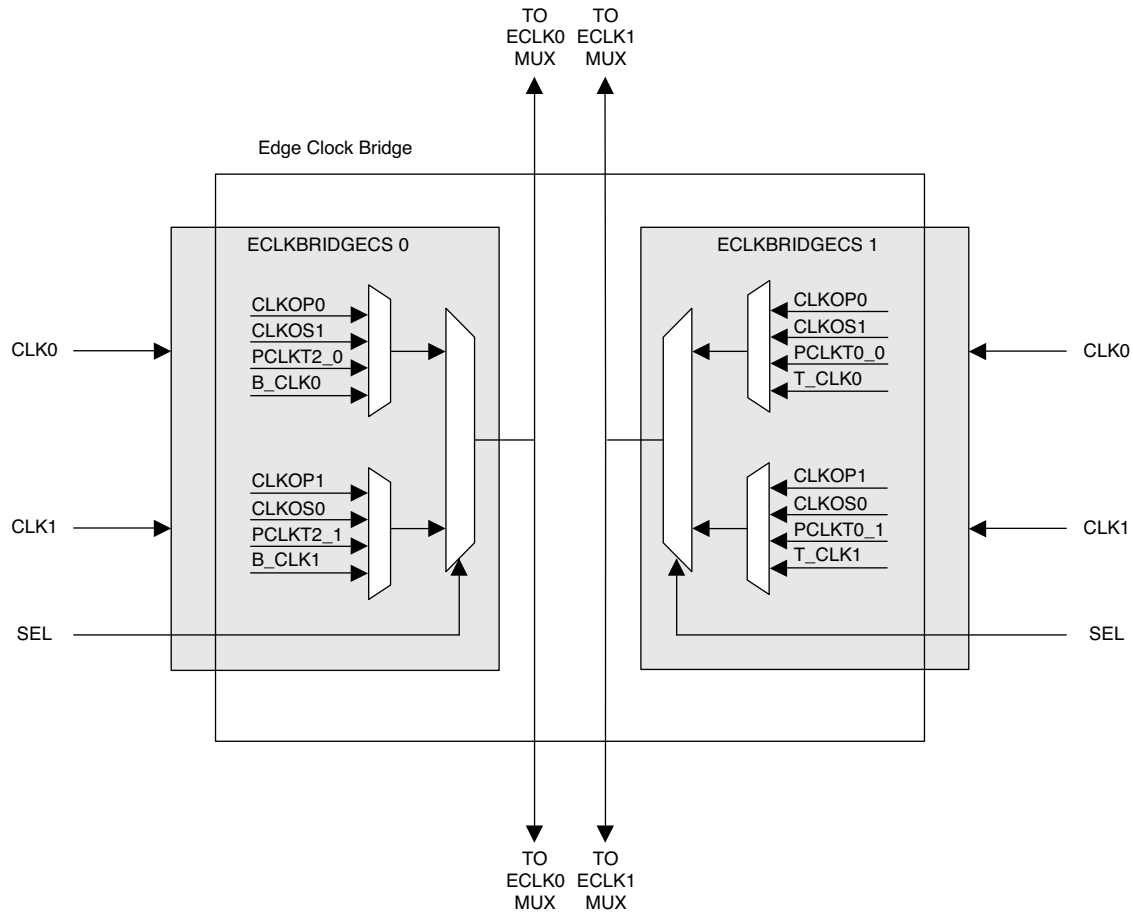
Figure 22. MachXO2 Edge Clock Bridge Sources and Connectivity
