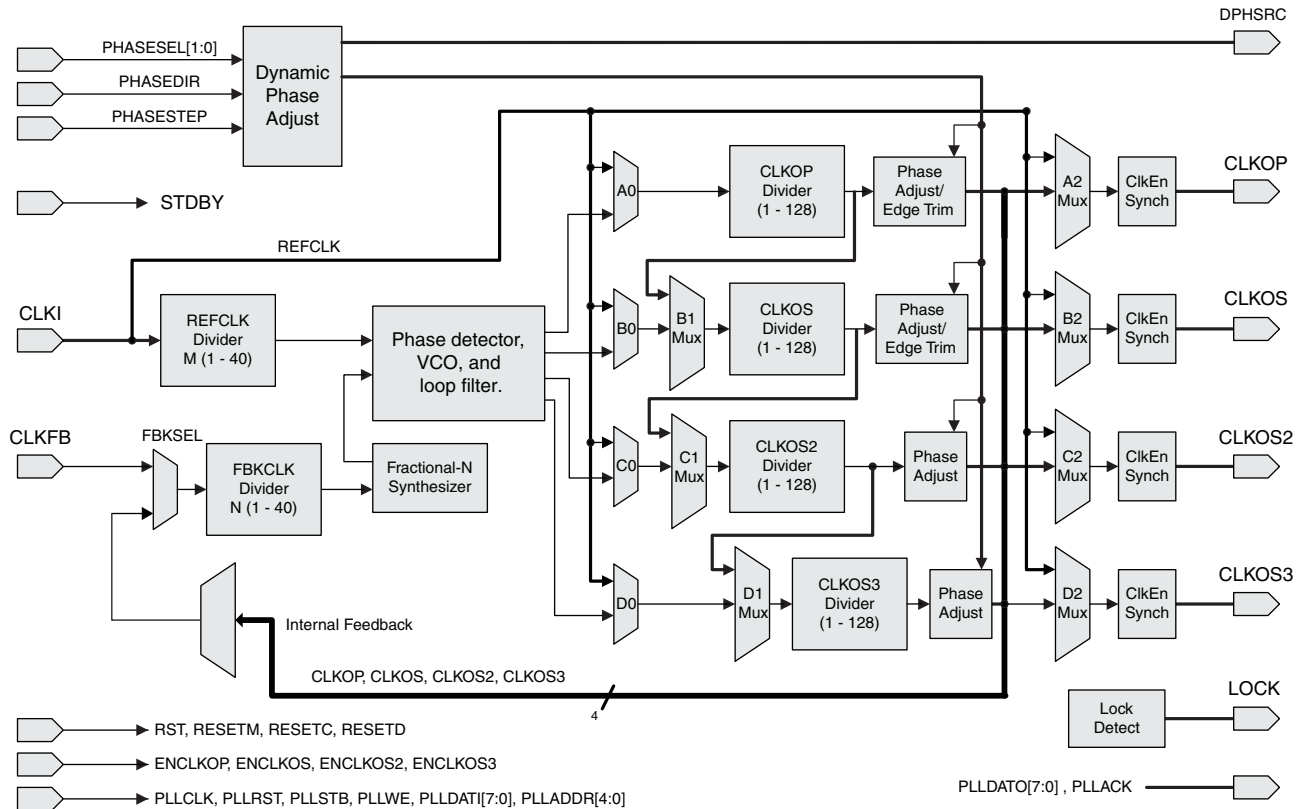
Figure 8. MachXO2 PLL Block Diagram
