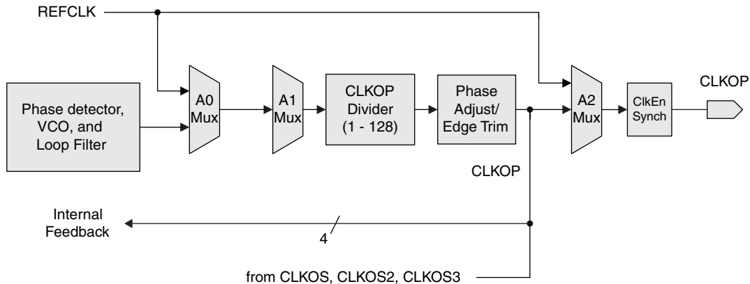
Figure 24. PLL CLKOP Output Section
