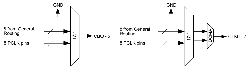
Figure 20. MachXO2 Primary Clock Muxes – MachXO2-256 and MachXO2-640
