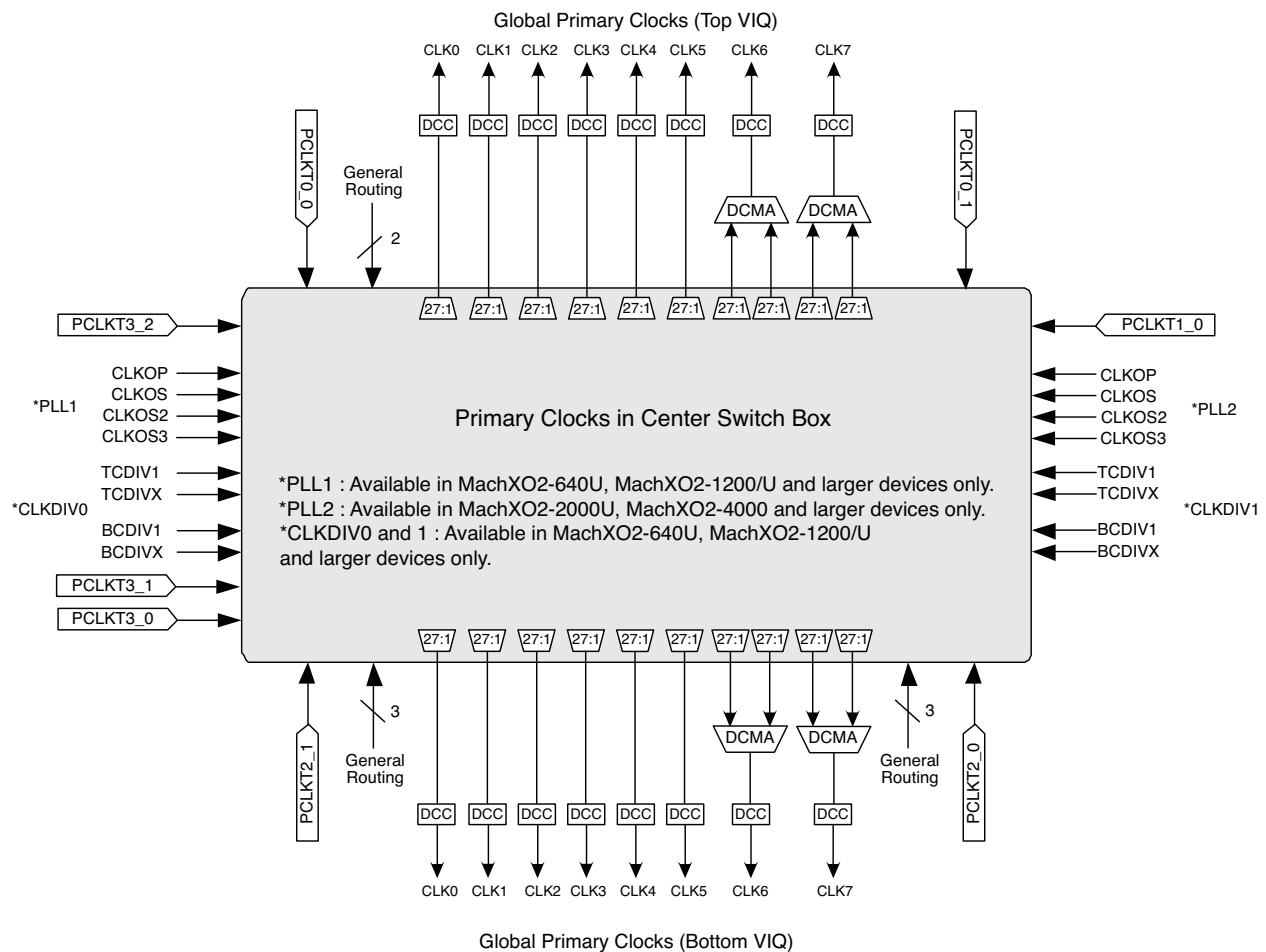
Figure 18. MachXO2 Primary Clock Sources and Distribution
