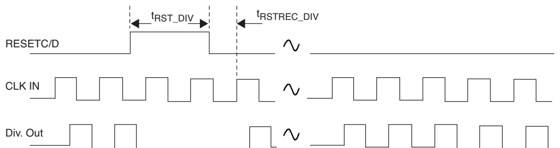
Figure 10. RESETC and RESETD Timing Diagram
